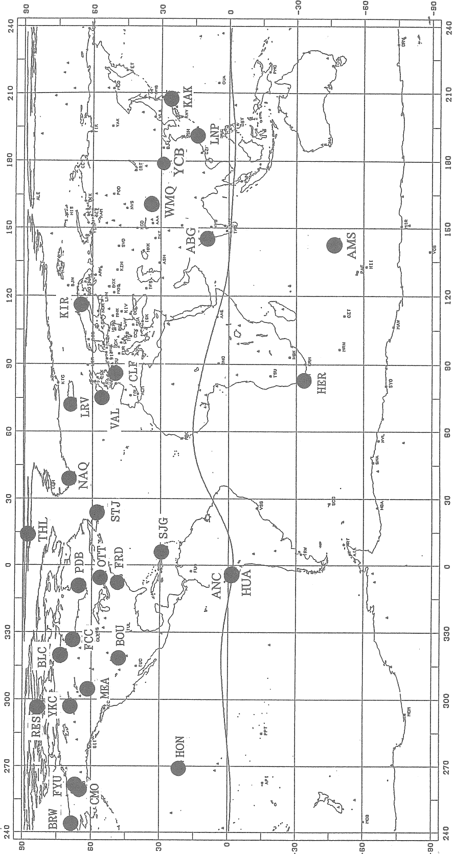
GEOMAGNETIC COORDINATE (1985. 0)
